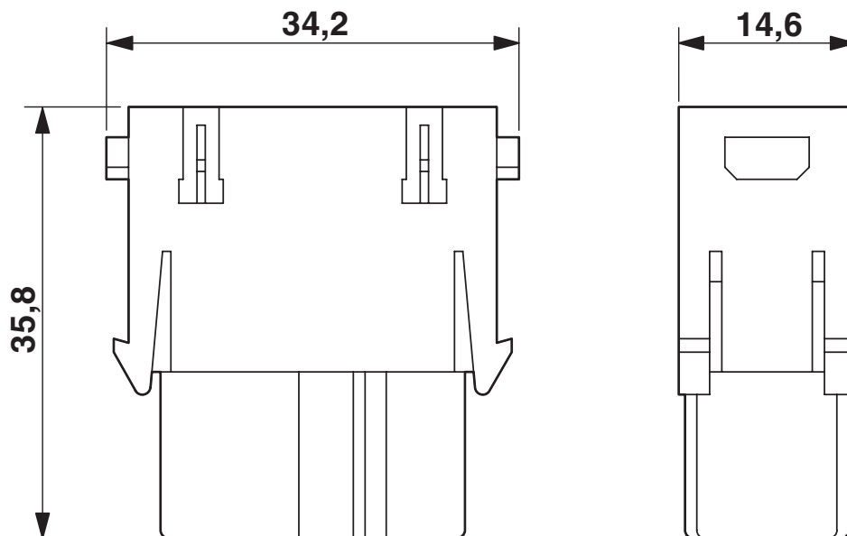
Dimensional drawing
